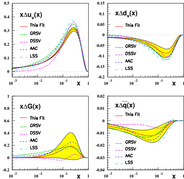
Figure 9: The NLO polarized parton distributions [157] at the input scale \mu = 2 GeV (solid line) compared to results obtained by GRSV (dashed-dotted line) [158], DSSV (long dashed-dotted line) [159], AAC (dashed line) [160], and LSS (long dashed line) [161]. The shaded areas represent the fully correlated 1\sigma error bands calculated by Gaussian error propagation; from Ref. [157].
