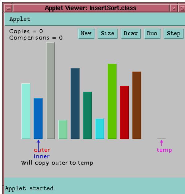
Figure 2.2: Insertion Sort
