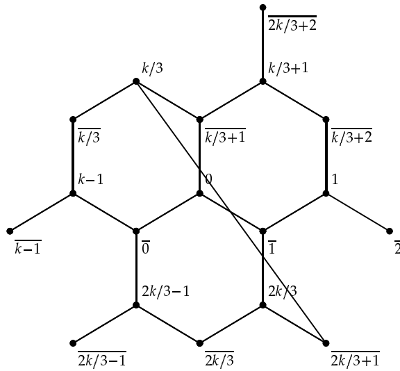
Figure 8.8: Neighborhood of 0 in CR(k, k/3 + 1) .
