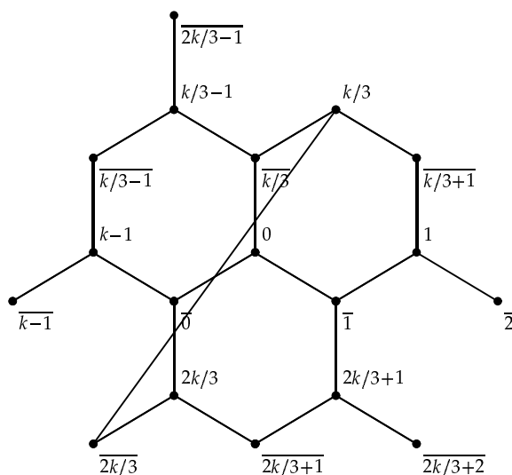
Figure 8.7: Neighborhood of 0 in \text{CR}(k, k/3) .
