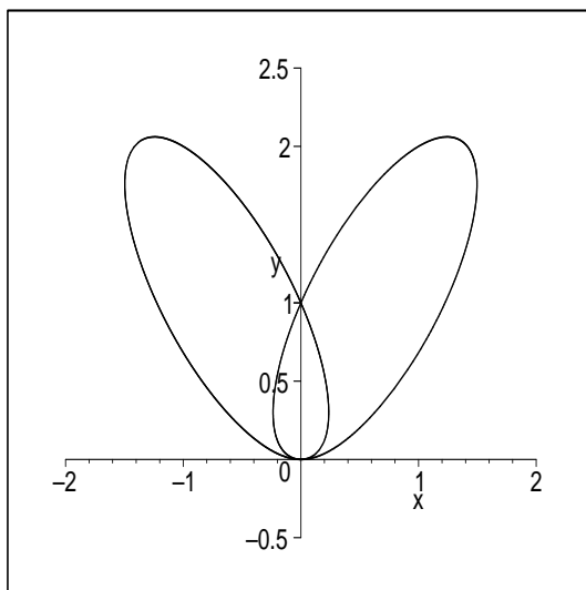
Figure 8.1: Tacnode curve
