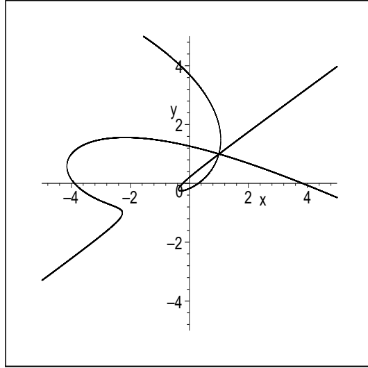
Figure 8.2: Quartic \mathcal{C}
