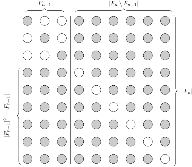
Fig. 1. Geometric proof of Theorem 3.3 for |F_1| = 3 .
